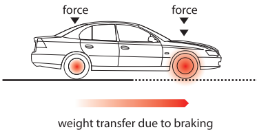
Electronic Brakeforce Distribution (EBD)
